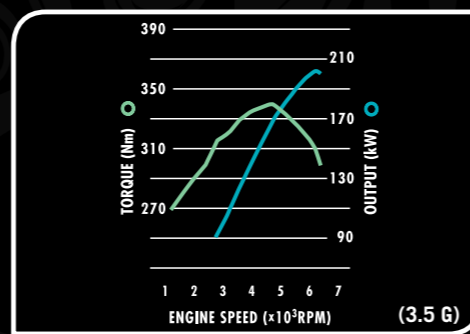
Performance for your convenience: 3.5-litre Dual VVT-i V6-engine with 275 PS (3.5 G) or the 2.4-litre VVT-i I4-engine with 170 PS (2.4 G and 2.4 X)
